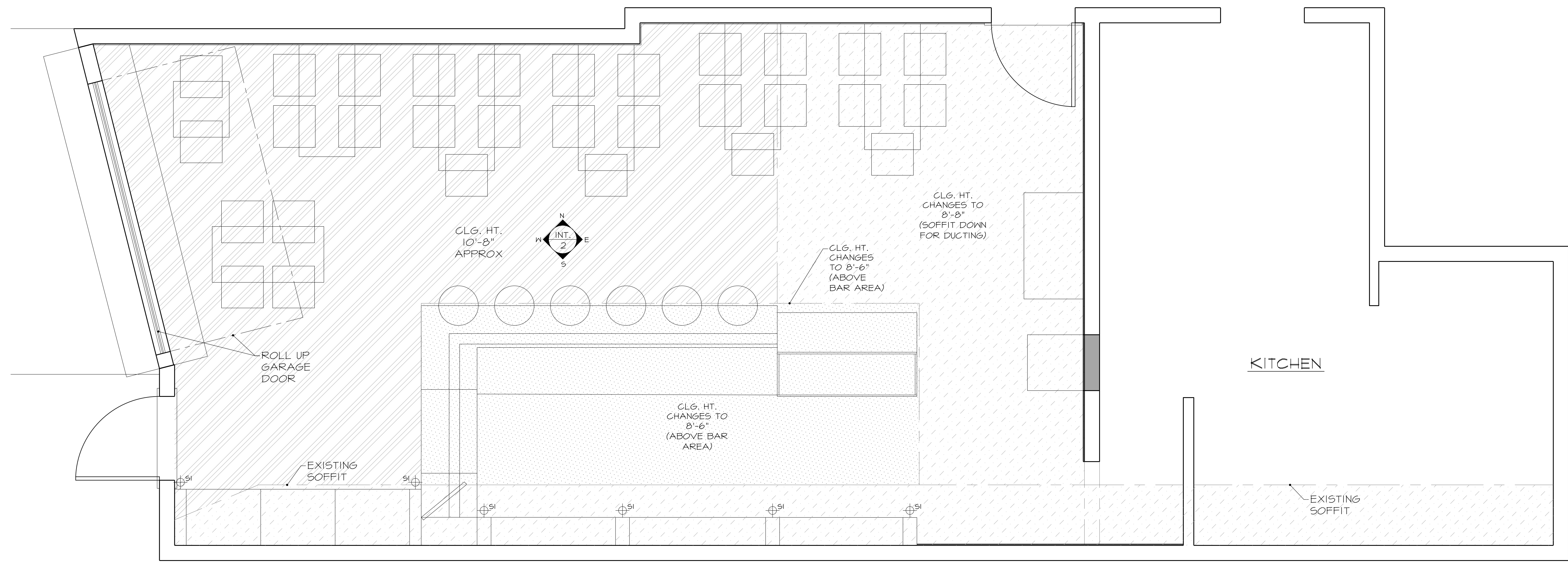
WORTHY TAPS & TACOS SCALE: 1/2"=1'-0" RCP
